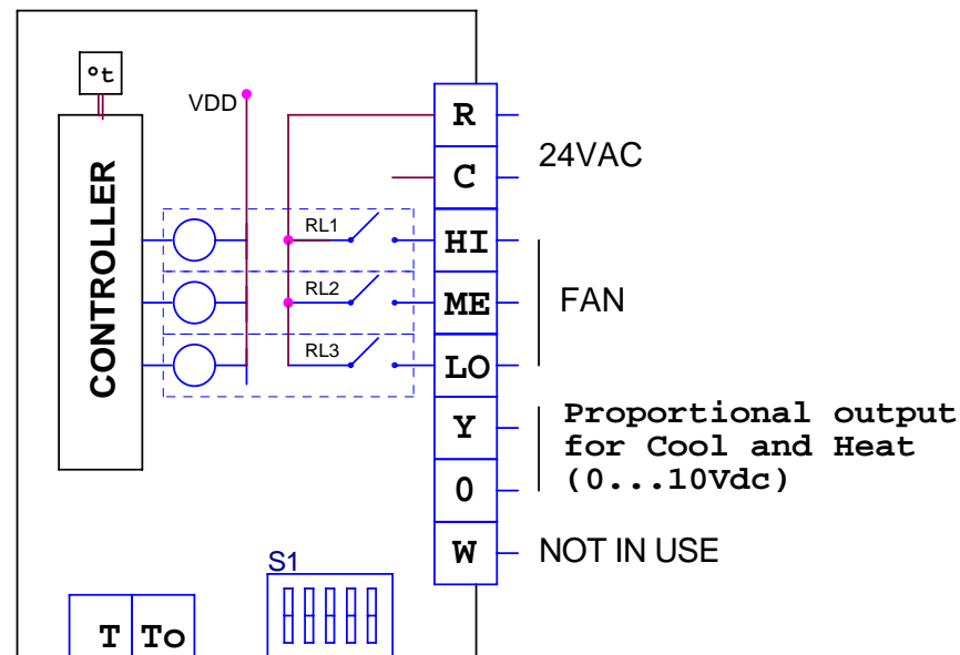
EXTERNAL SENSOR
